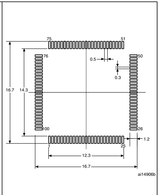
Figure 70. Recommended footprint (1)(2)
